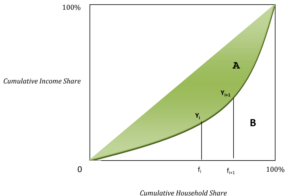
Lorenz Curve
